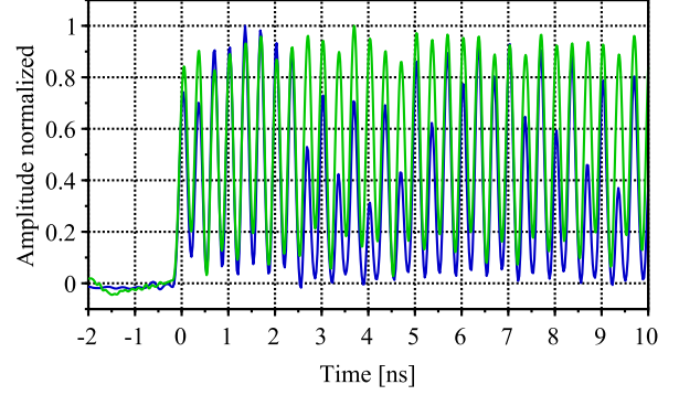
Figure 7: Start of a long 3 GHz macropulse measured by VFCT (blue) and cathode laser intensity (green).
