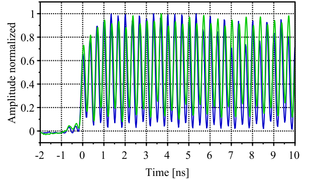
Figure 8: Start of a long 3 GHz macropulse measured by VFCT (blue) and cathode laser intensity (green) after laser position tuning.
